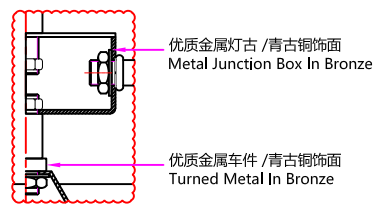
A 部细节图/Part A Details
