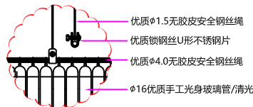
B 区放大图/Part B Details
