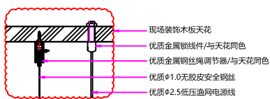
A 部细节图/Part A Details
