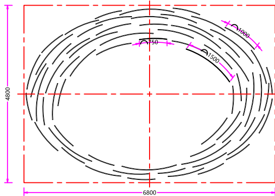
俯视图/Vertical View
